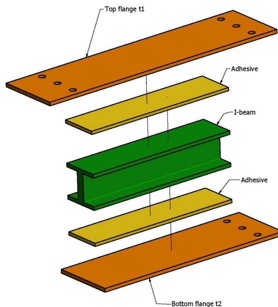
Figure 1 Beam assembly exploded view
