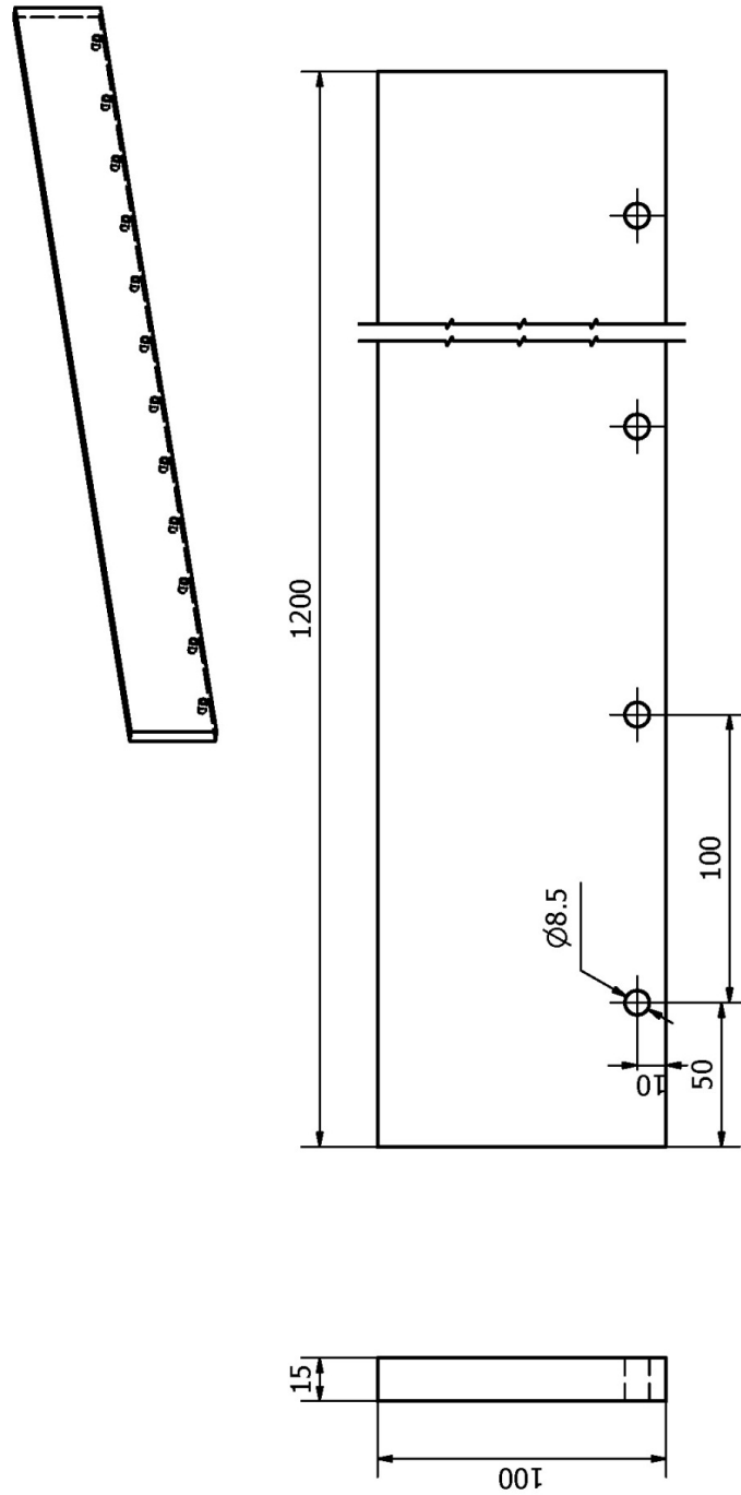
Figure 8 I-Beam mould 2 geometry
