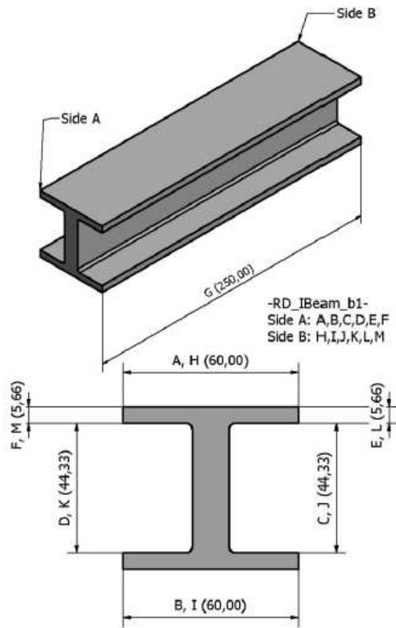
Figure 2 I-Beam geometrical dimensions
