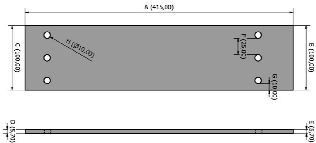
Figure 3 Flange t1
