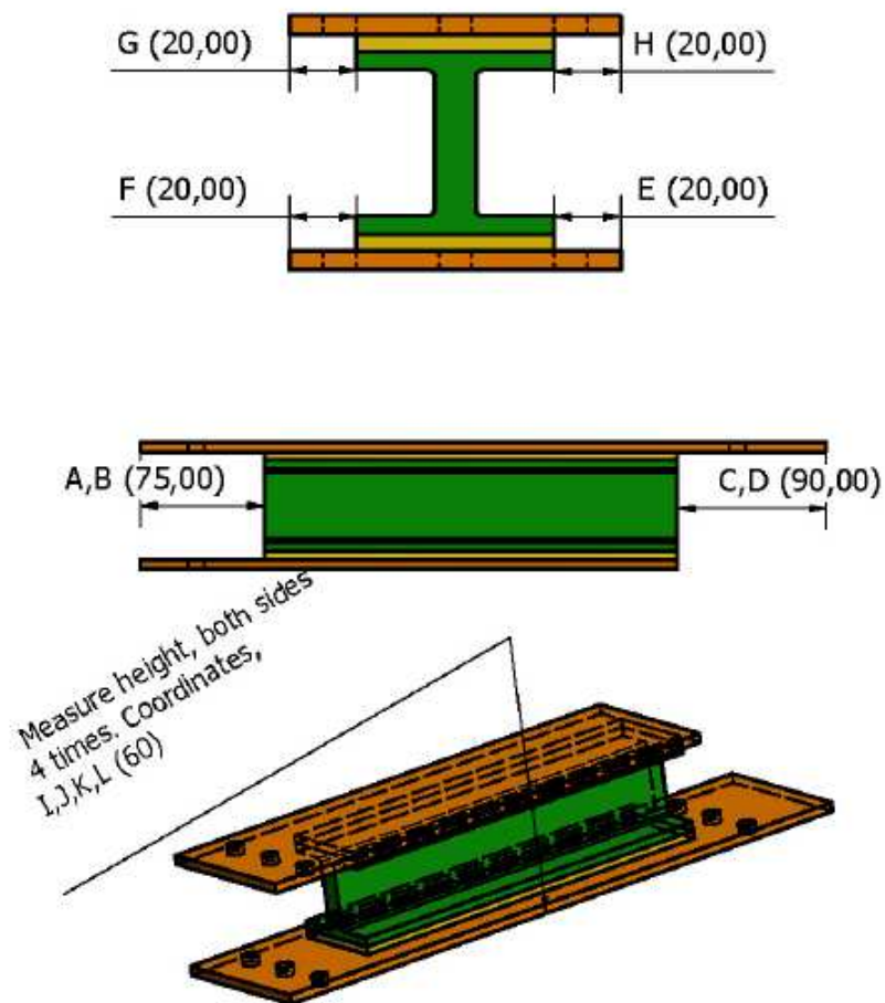
Figure 5 Beam assembly geometrical dimensions
