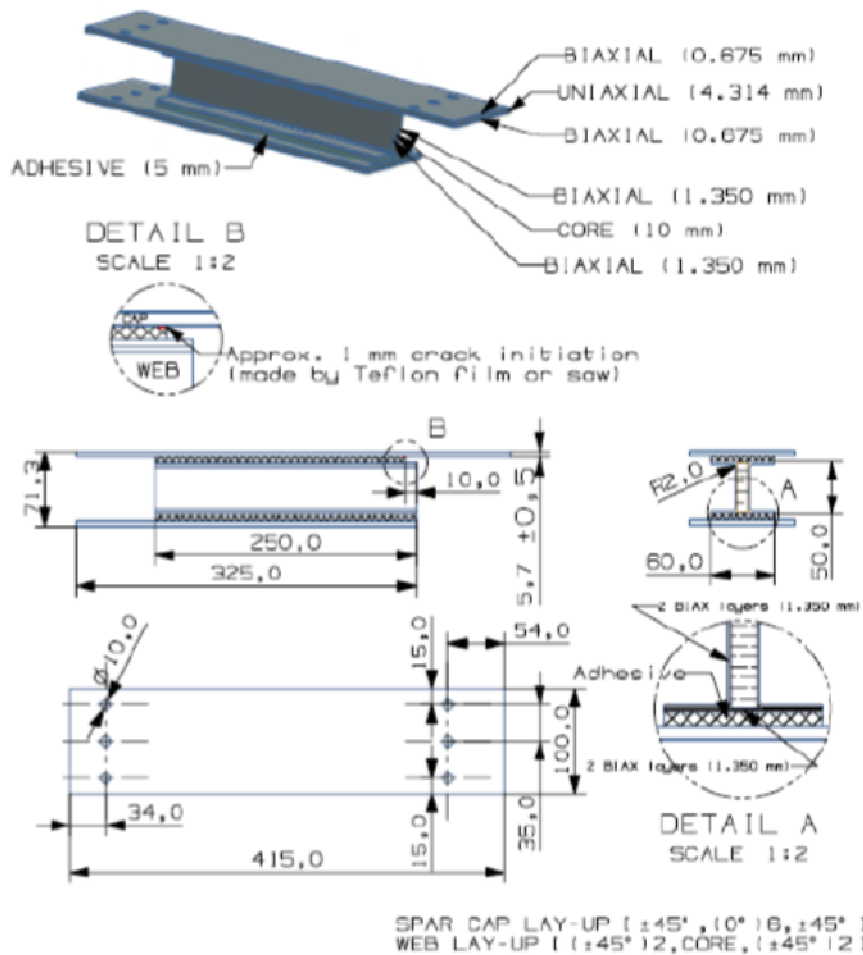
Figure 6 I-Beam geometry & stacking sequence
