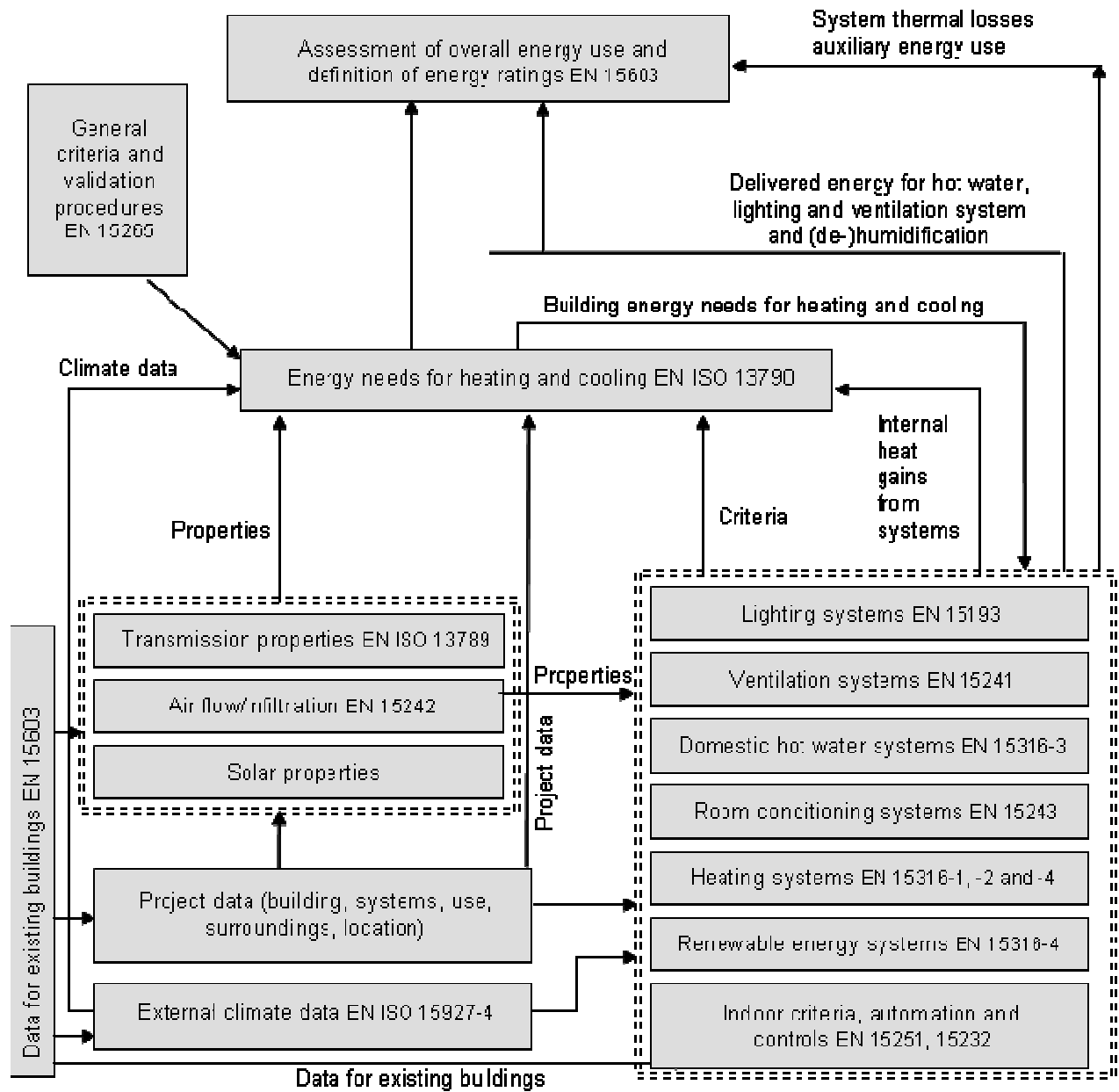
Figure 4 – Outline of linkage diagram for the building part
