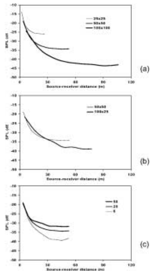
Figure 7.5: Effect of Square Size, Aspect Ratio and Height. The Basic Square Configuration is 50x50m, 20m High, and Absorption Coefficient 0.1.
