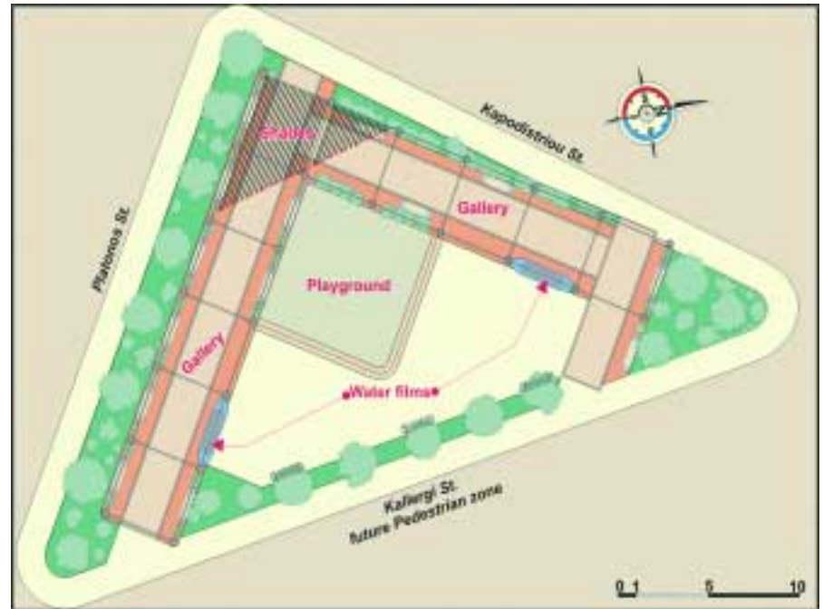
Figure 8.13: Plan view of the design proposal.
