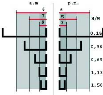
Figure 3.1: Shadow path overlapped to the sections of NS oriented streets.
