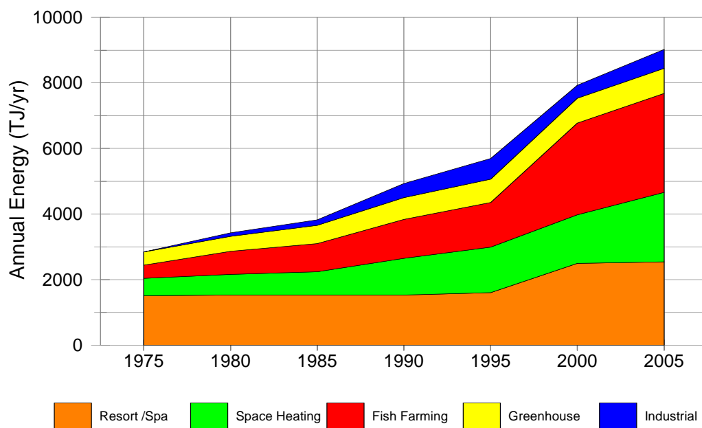
FIGURE 6. Direct-Use growth in the United States.
