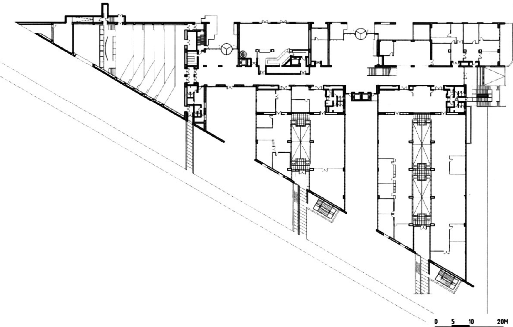
KATOVI DEOTEIOY GROUND FLOOR PLAN
