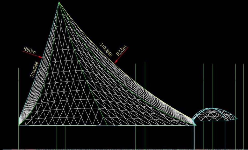
ELEVATION A OF PROPOSED STRUCTURE
