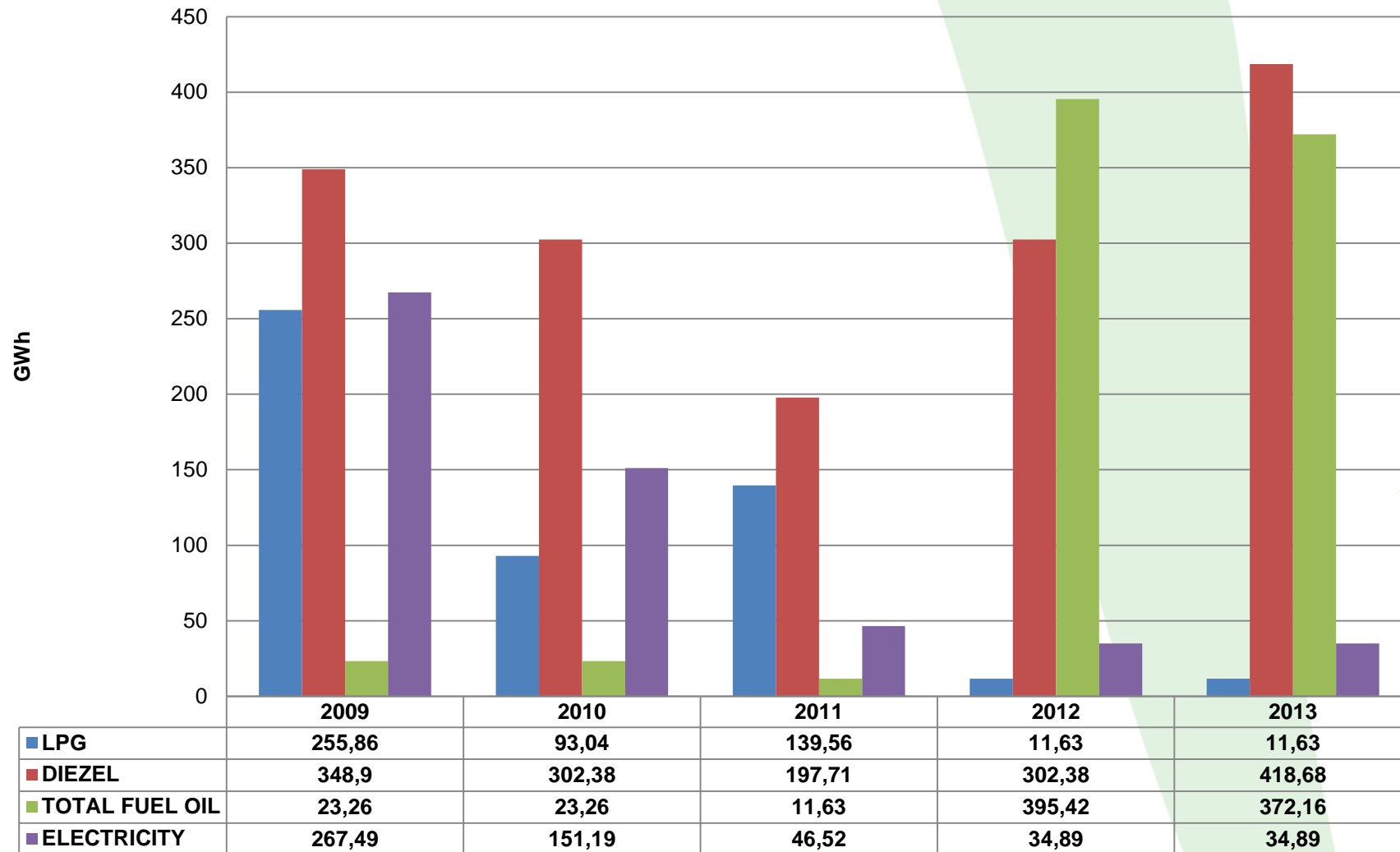
Final energy consumption in Mining and quarrying
