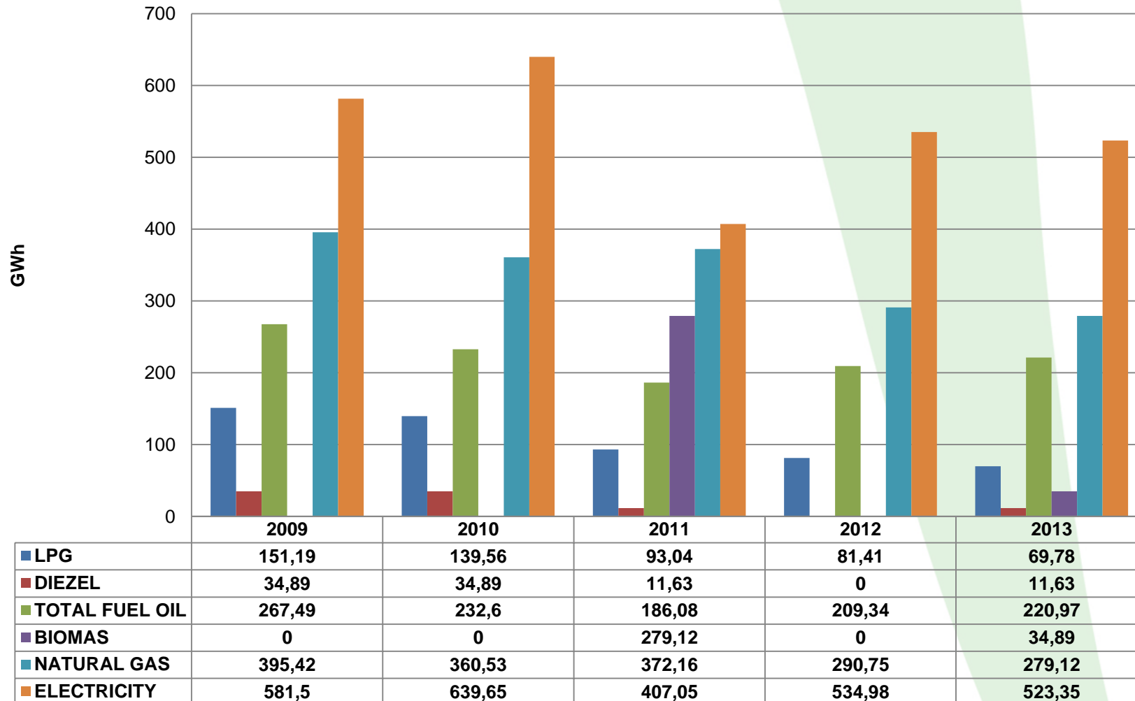
Final energy consumption in paper and paper products
