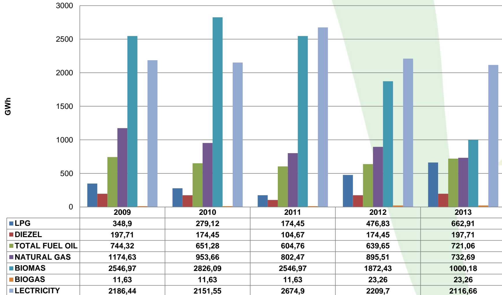
Final energy consumption in Food, beverage and tobacco
