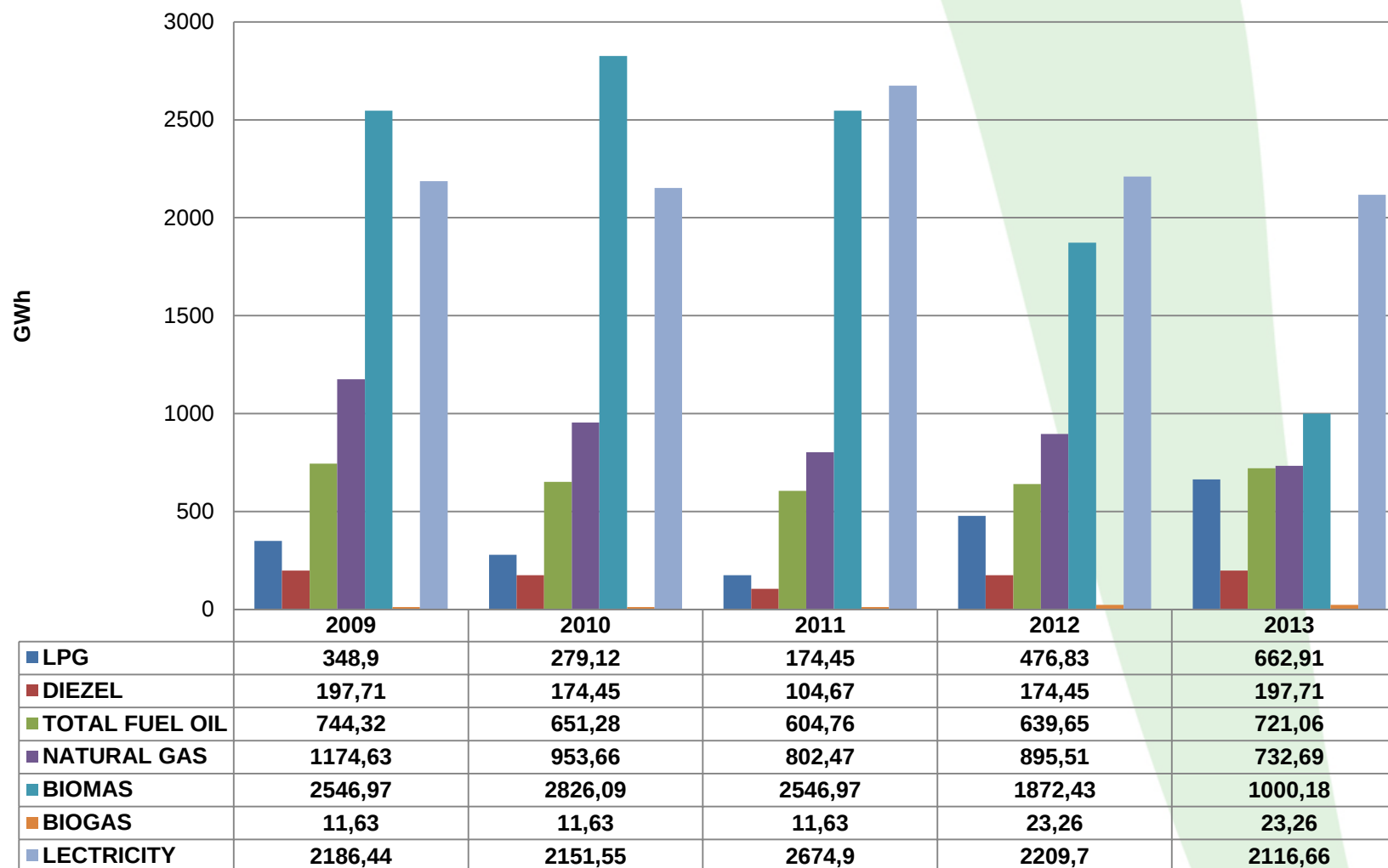
Final energy consumption in Food, beverage and tobacco
