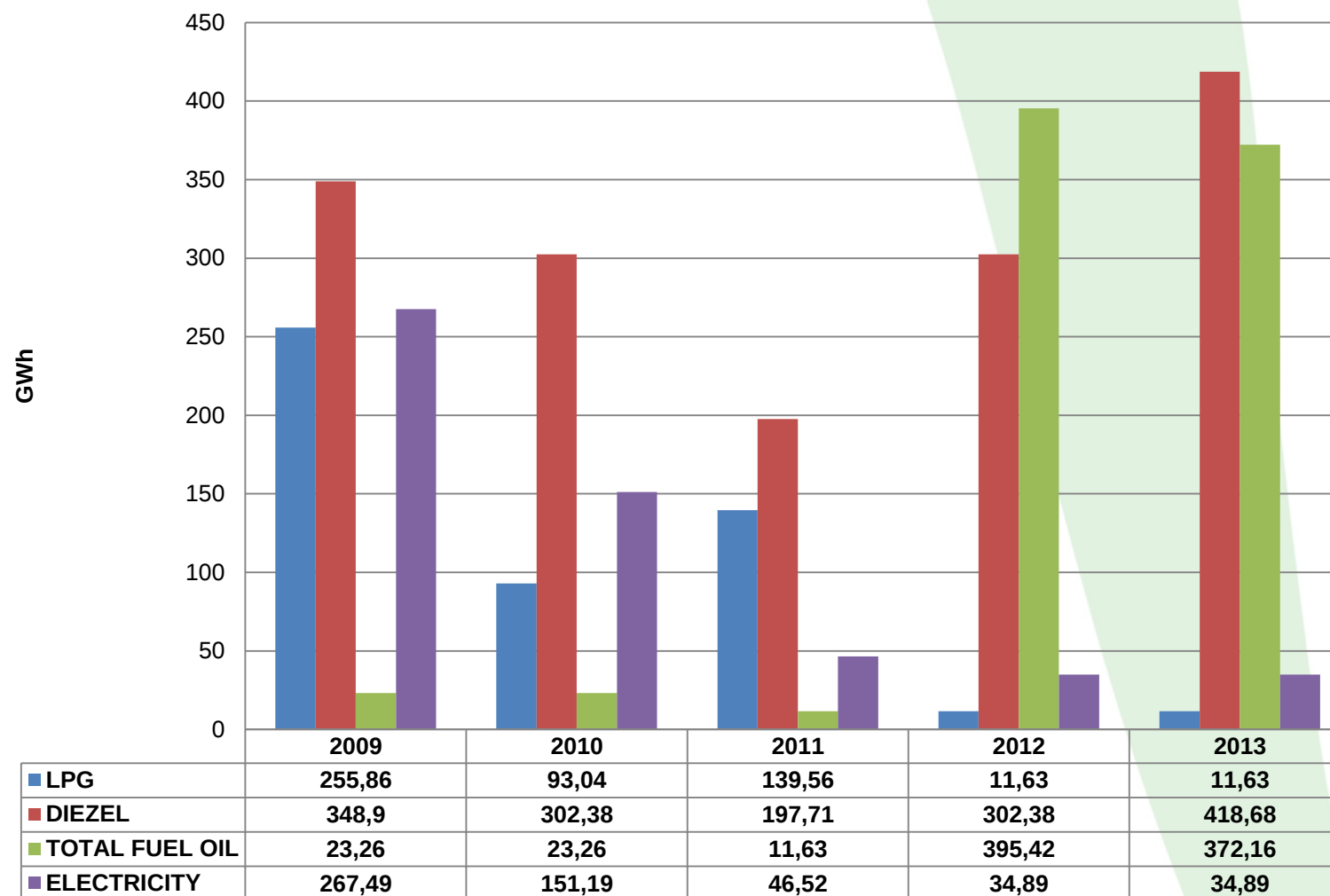
Final energy consumption in Mining and quarrying
