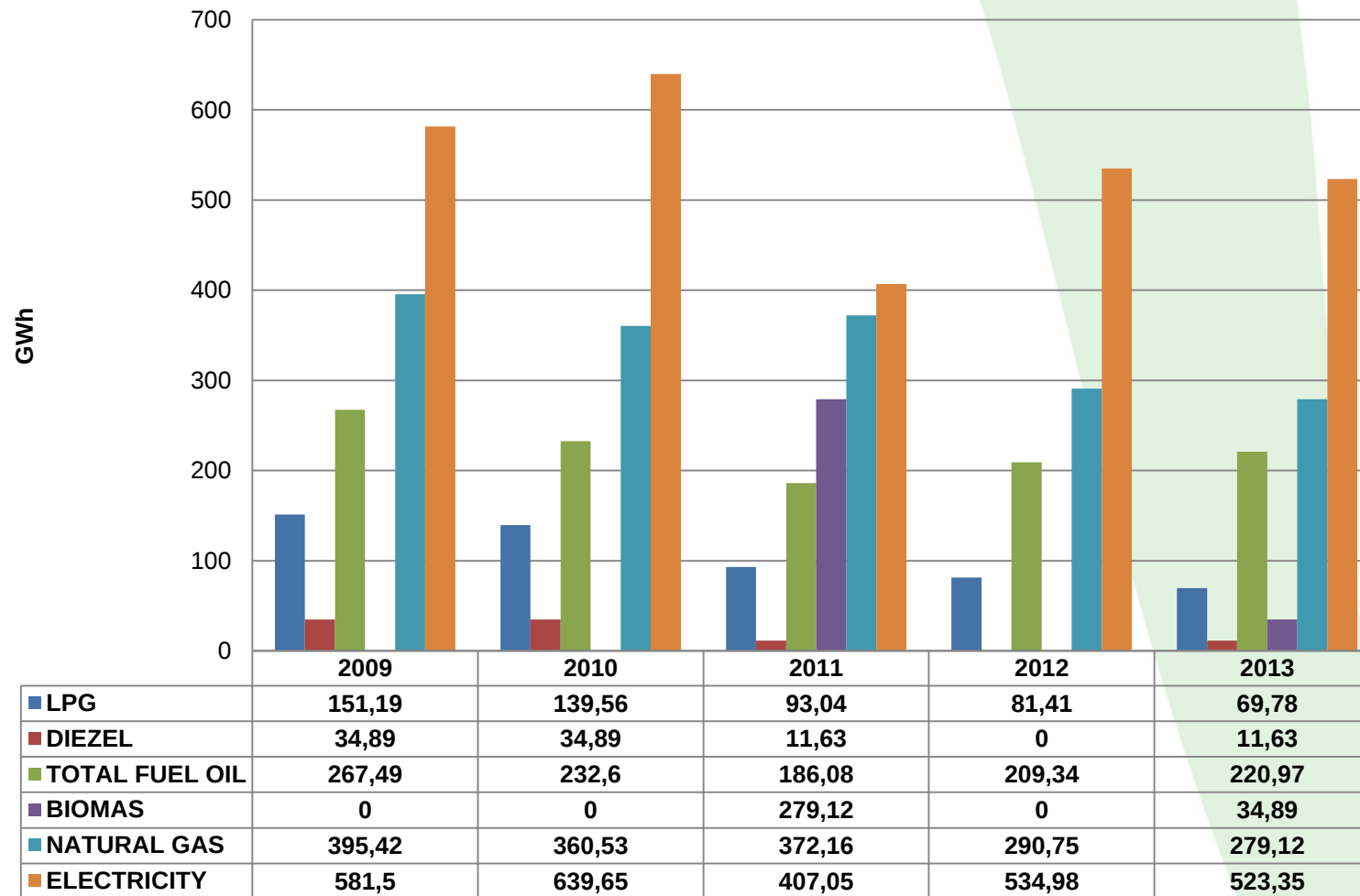
Final energy consumption in paper and paper products
